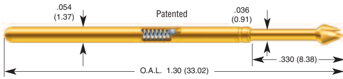
POGO-25I POGO-25I-S
